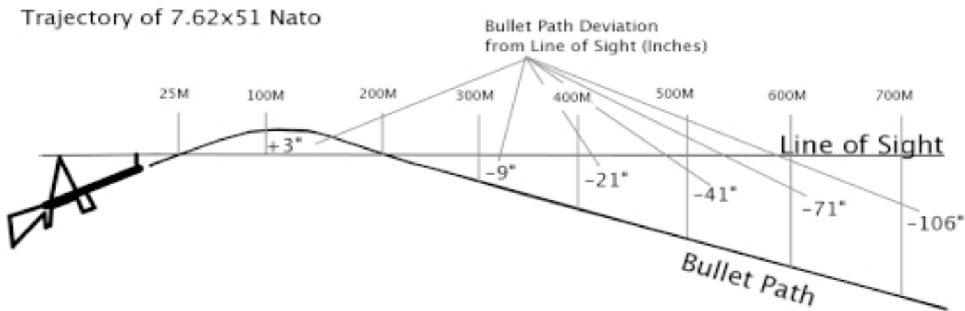
Figure 30. 7.62x51 Ball Trajectory
